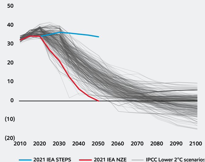
Global CO 2 emissions (GT CO 2 )
